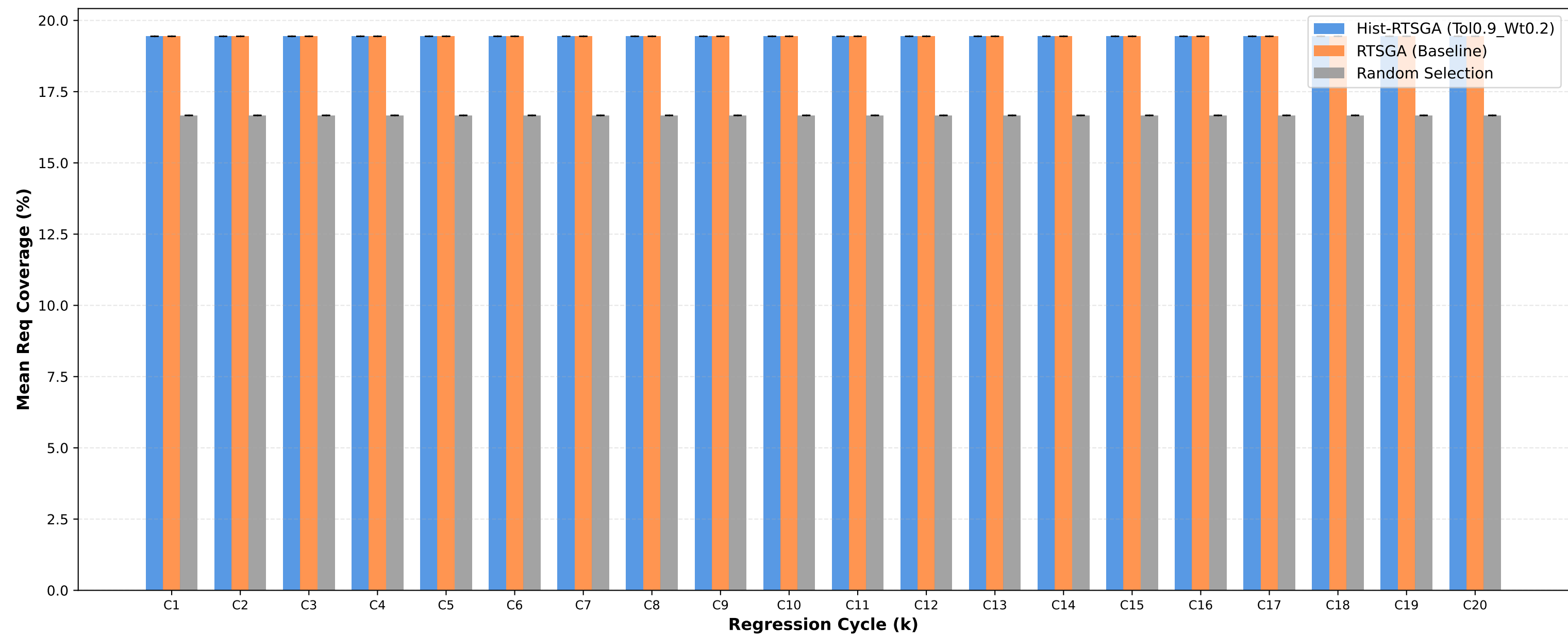
Req Coverage: Tol0.9_Wt0.2 vs RTSGA vs Random
