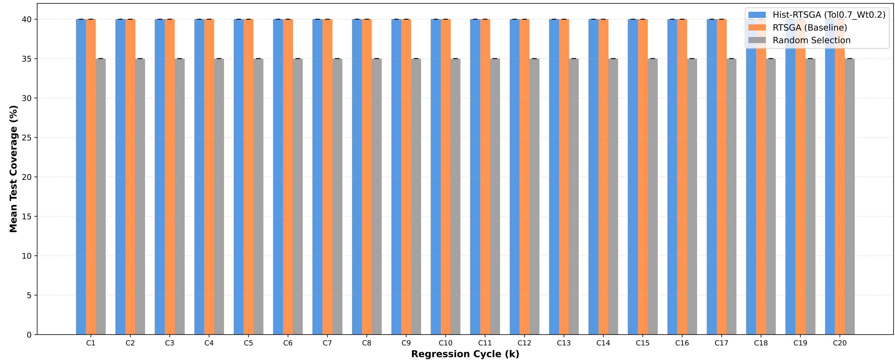
Test Coverage: Tol0.7_Wt0.2 vs RTSGA vs Random
