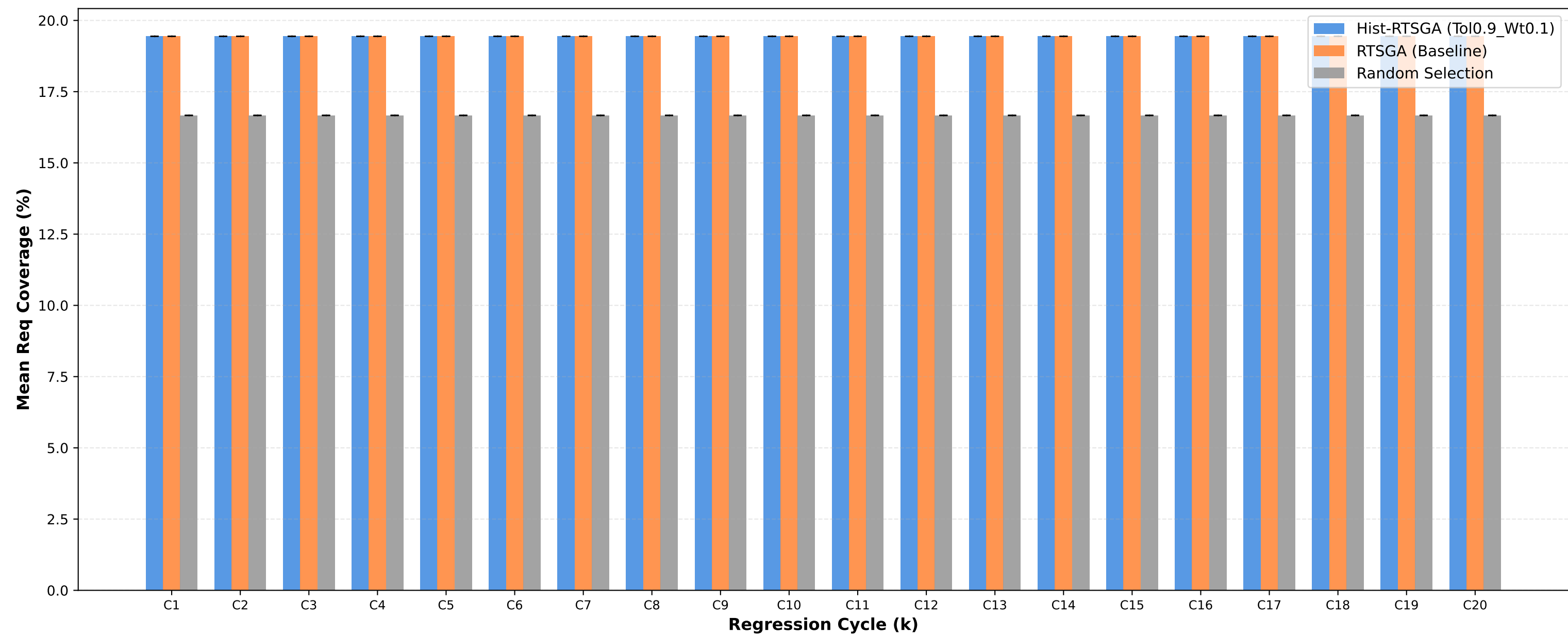
Req Coverage: Tol0.9_Wt0.1 vs RTSGA vs Random
