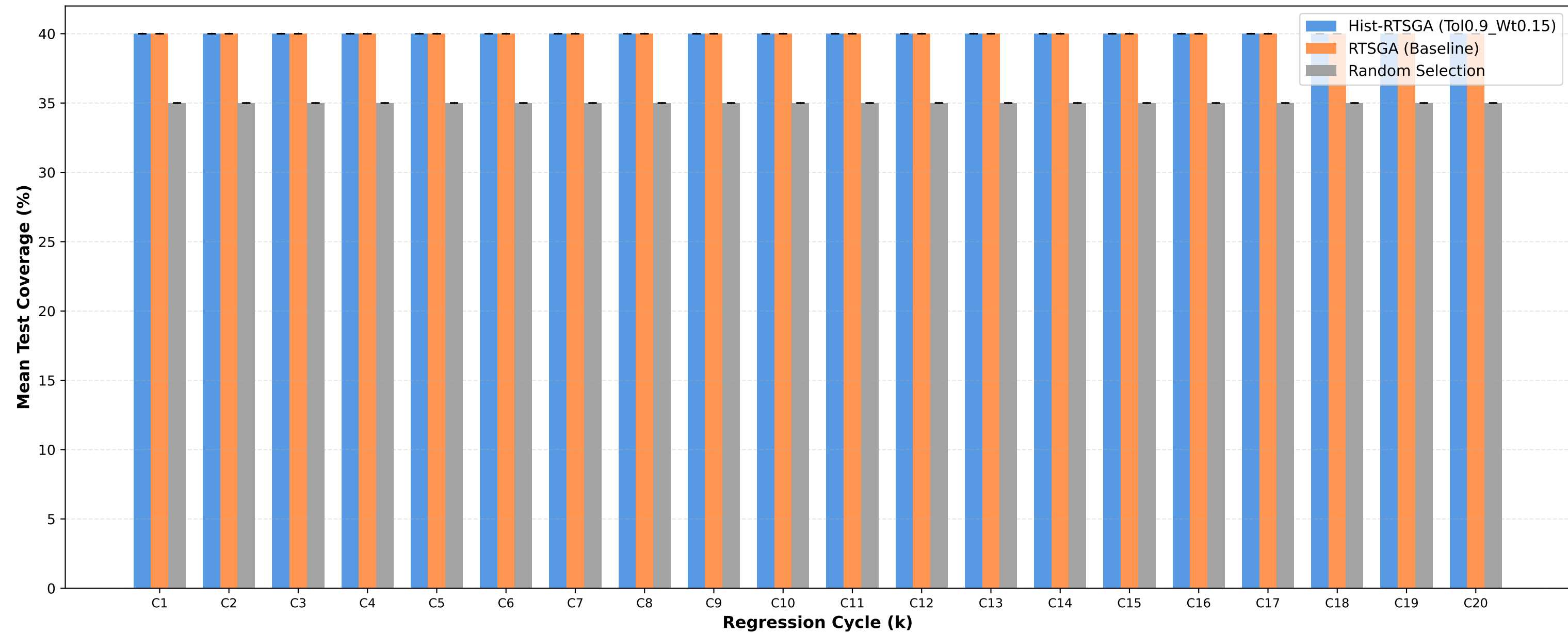
Test Coverage: Tol0.9_Wt0.15 vs RTSGA vs Random
