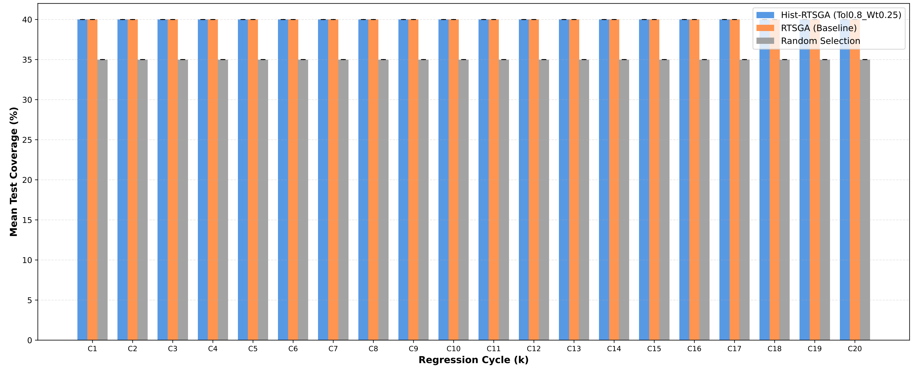
Test Coverage: Tol0.8_Wt0.25 vs RTSGA vs Random
