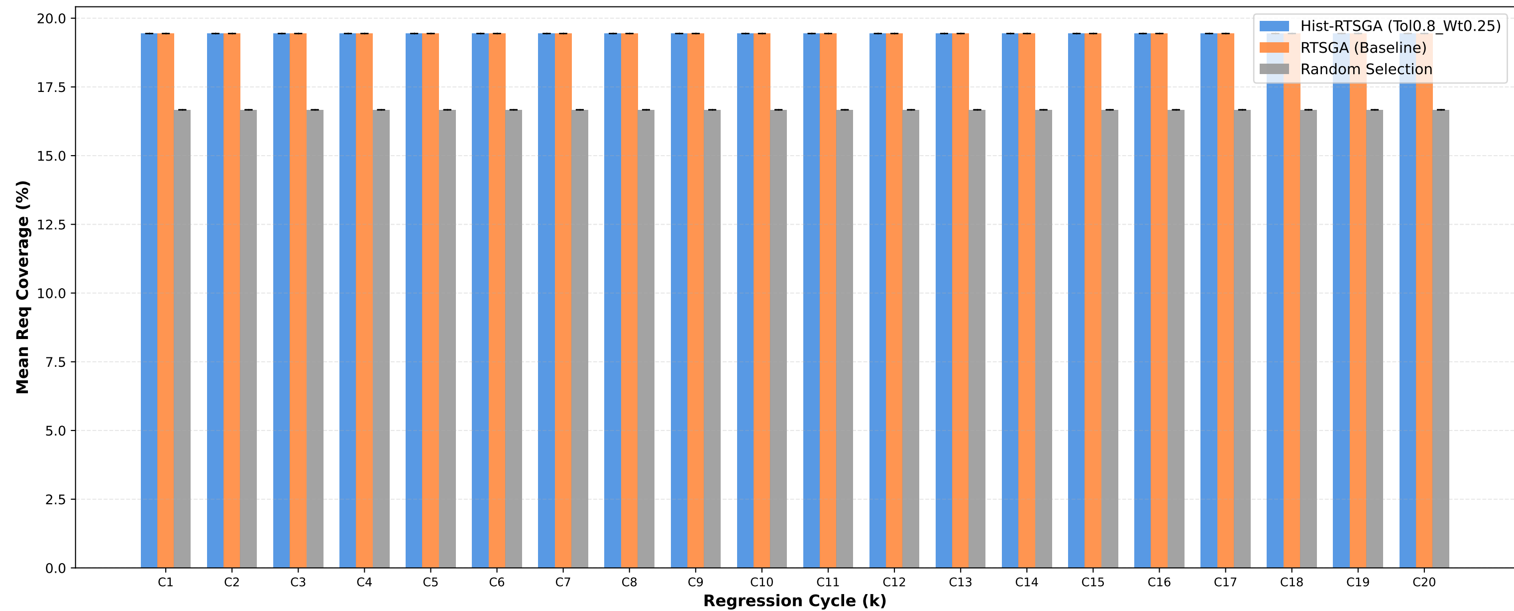
Req Coverage: Tol0.8_Wt0.25 vs RTSGA vs Random
