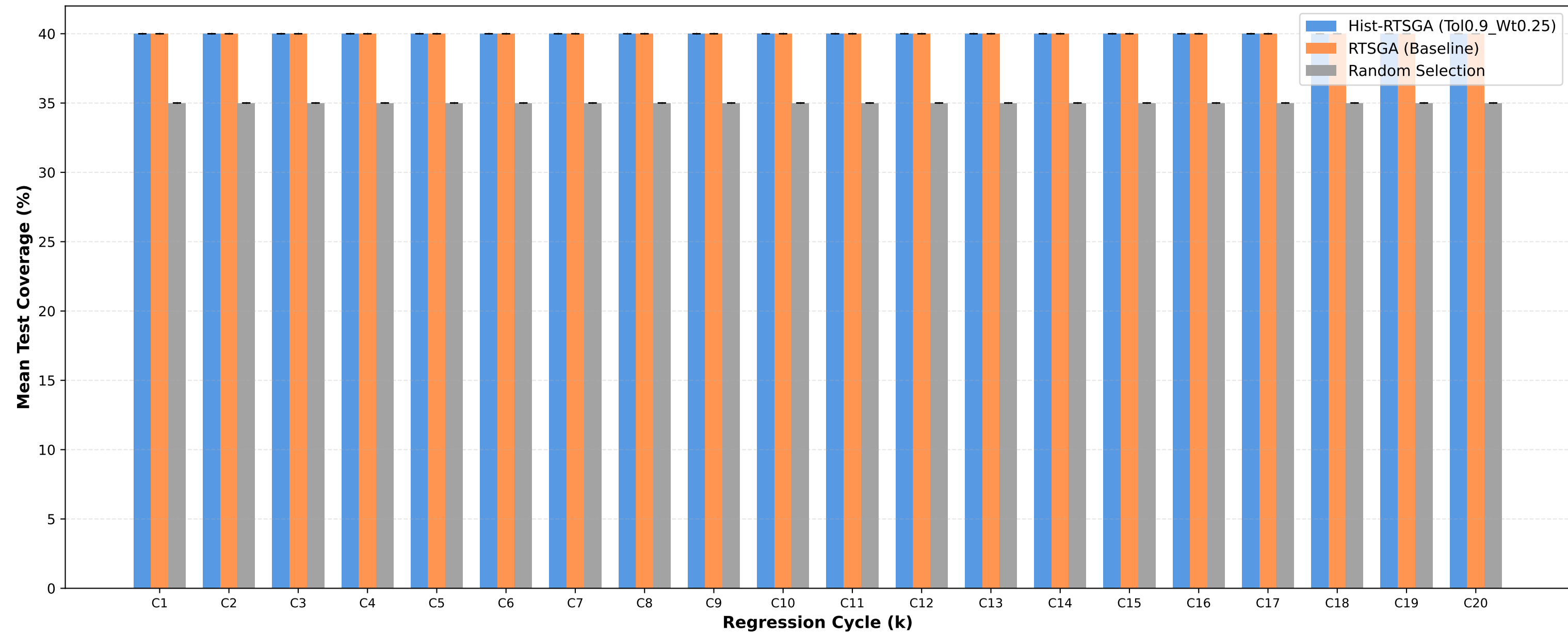
Test Coverage: Tol0.9_Wt0.25 vs RTSGA vs Random
