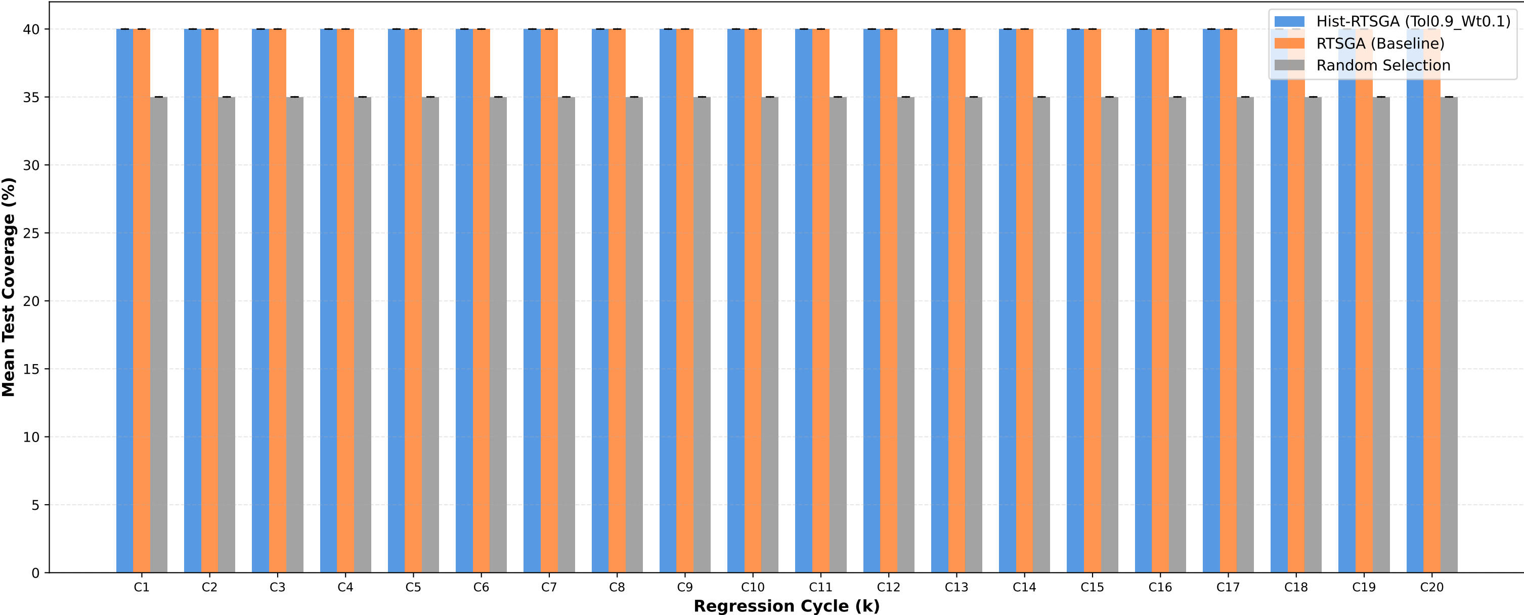
Test Coverage: Tol0.9_Wt0.1 vs RTSGA vs Random
