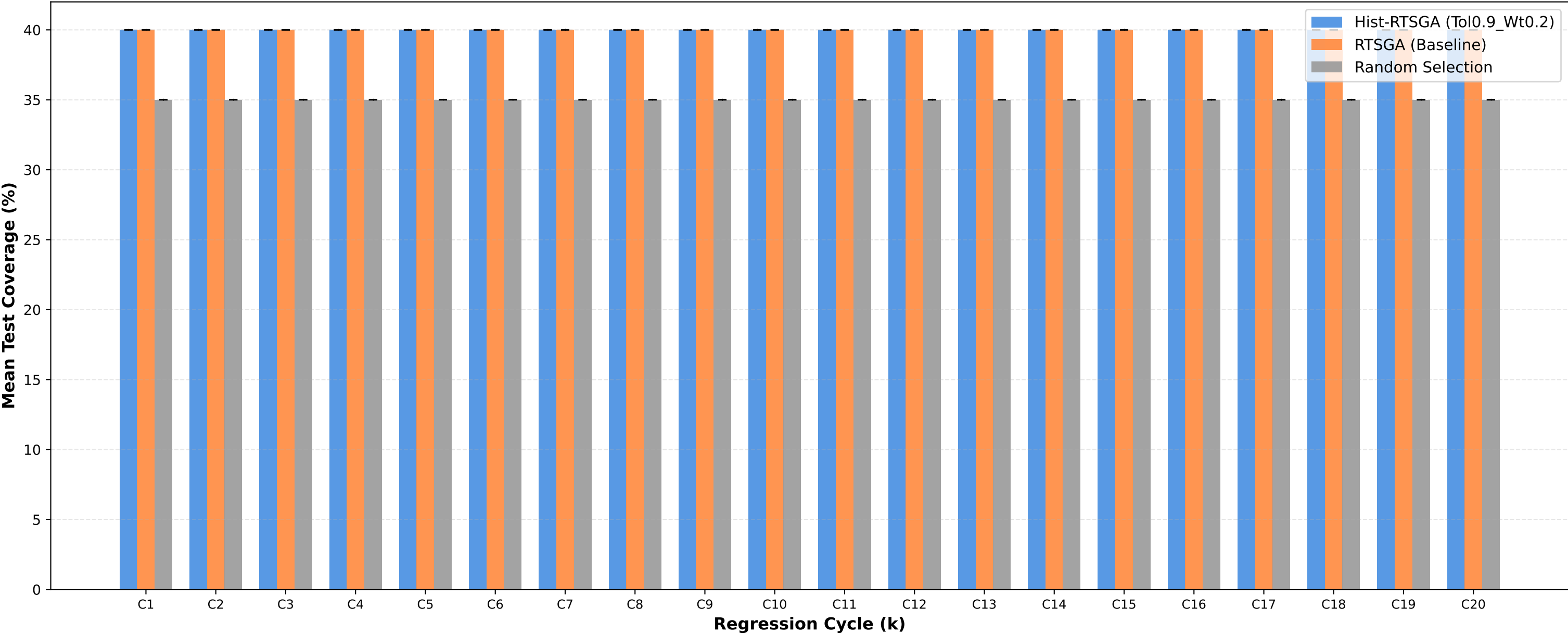
Test Coverage: Tol0.9_Wt0.2 vs RTSGA vs Random
