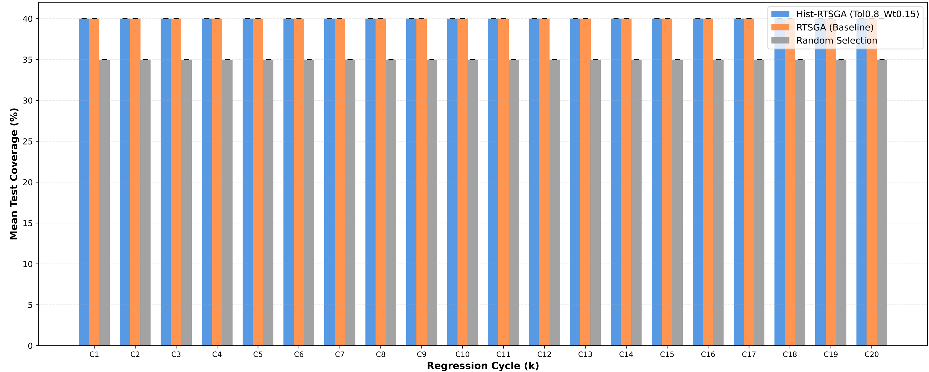
Test Coverage: Tol0.8_Wt0.15 vs RTSGA vs Random
