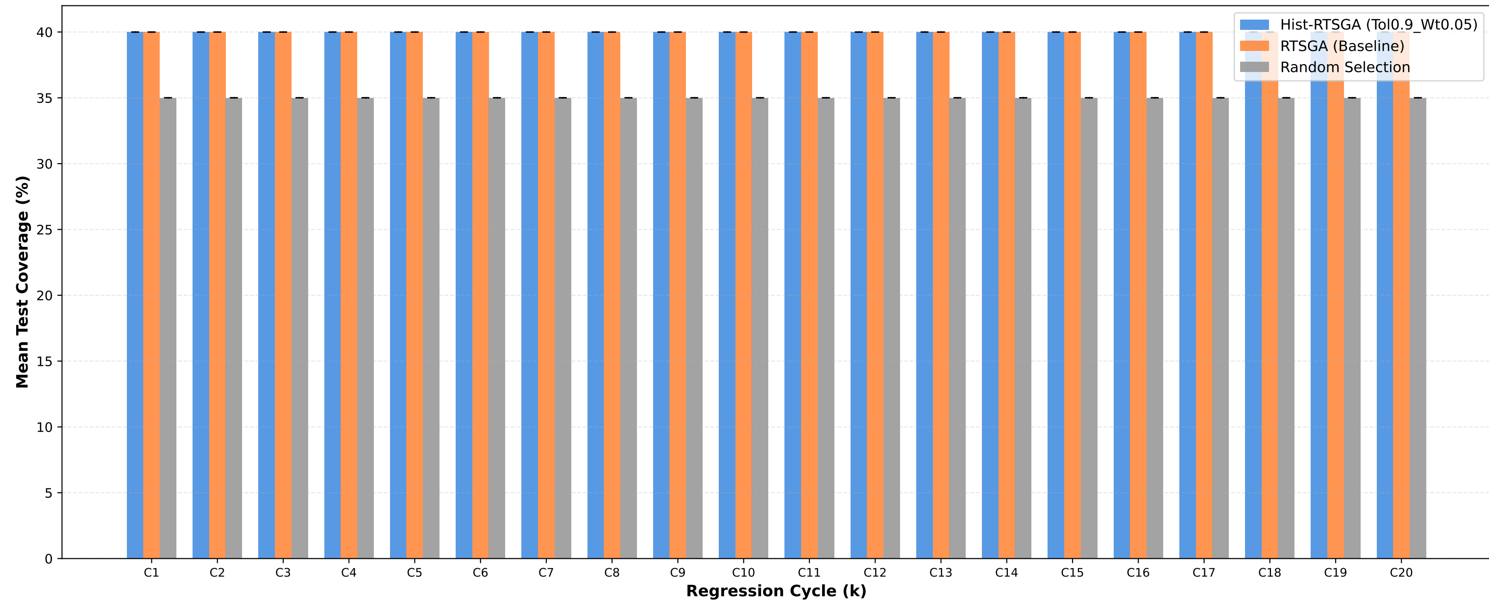
Test Coverage: Tol0.9_Wt0.05 vs RTSGA vs Random
