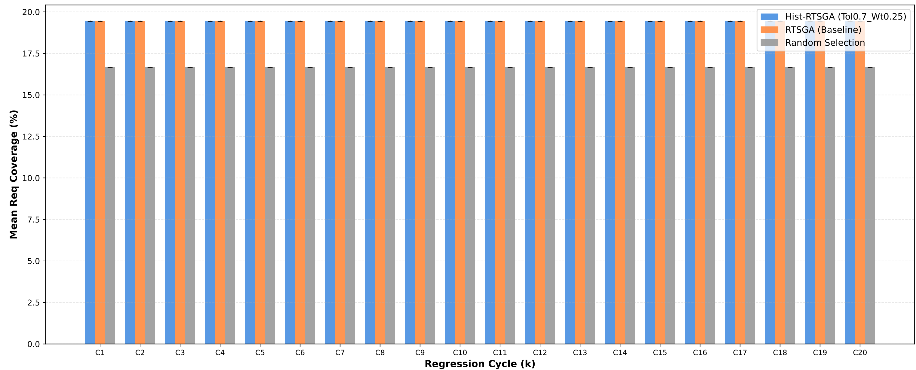
Req Coverage: Tol0.7_Wt0.25 vs RTSGA vs Random
