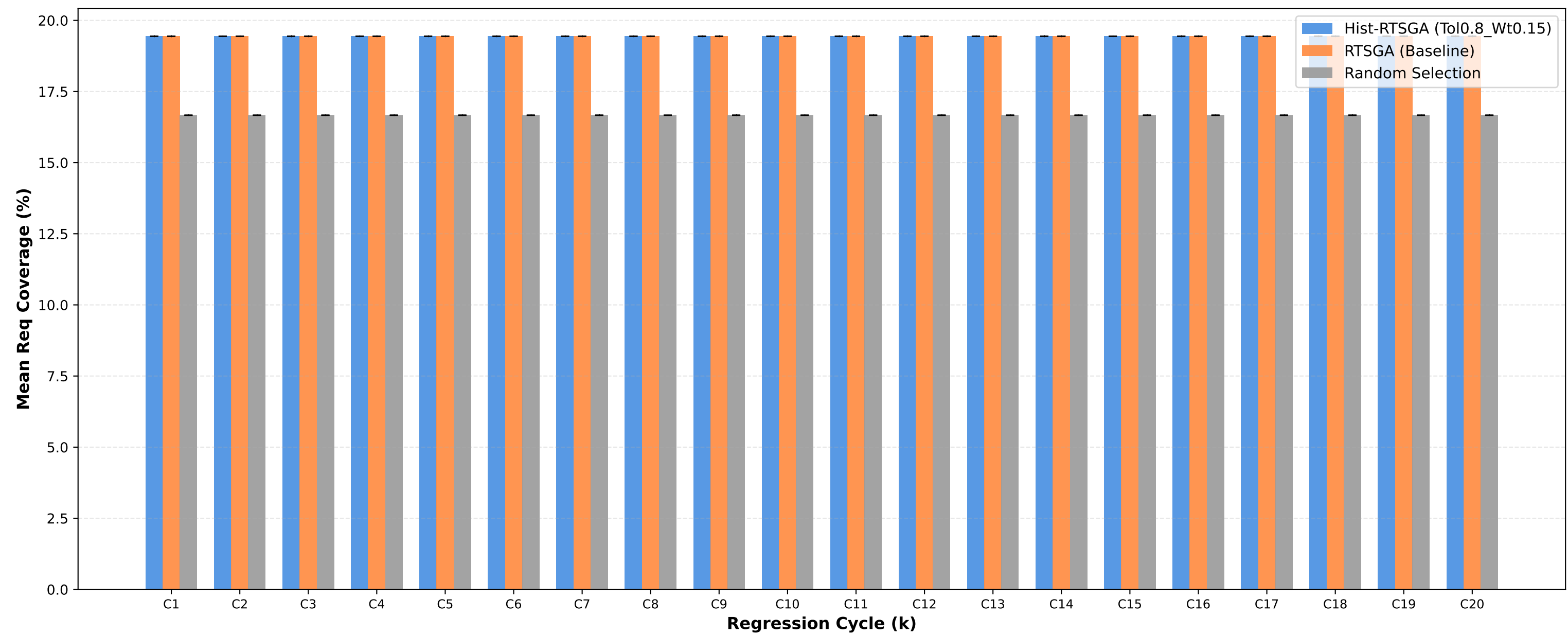
Req Coverage: Tol0.8_Wt0.15 vs RTSGA vs Random
