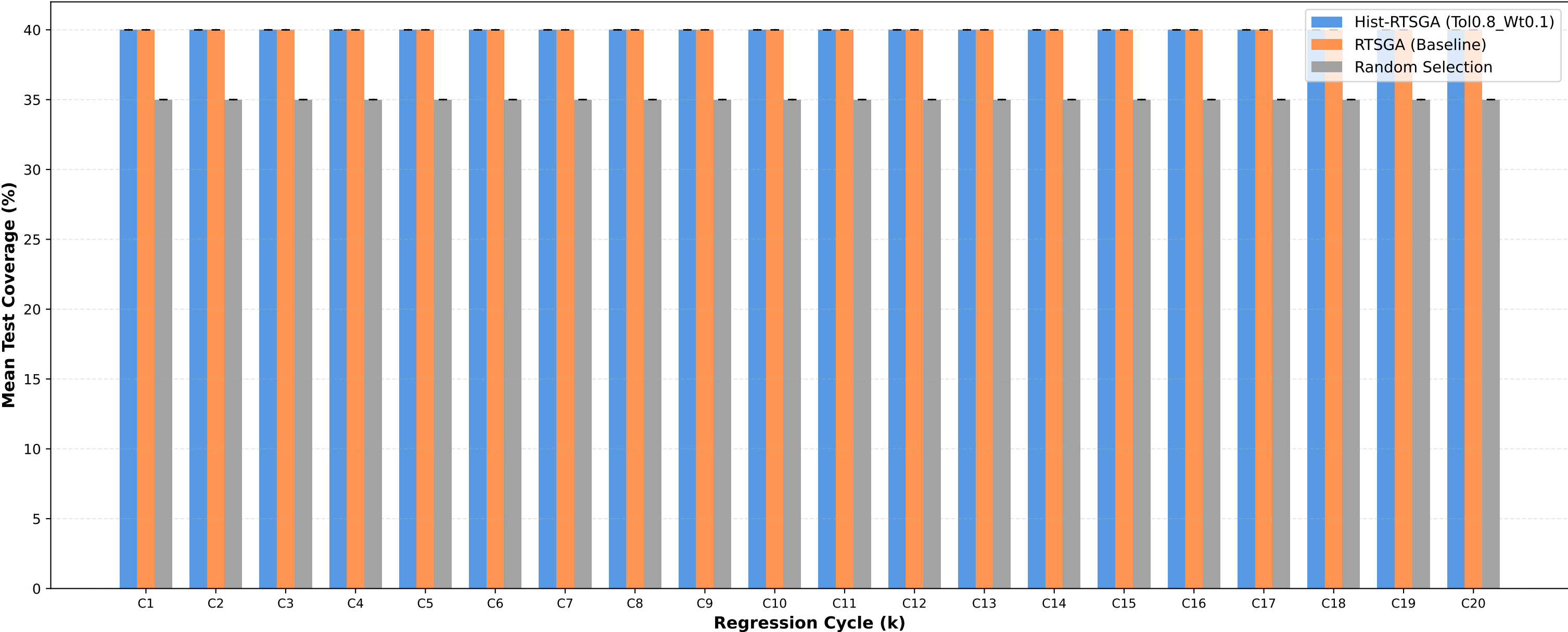
Test Coverage: Tol0.8_Wt0.1 vs RTSGA vs Random
