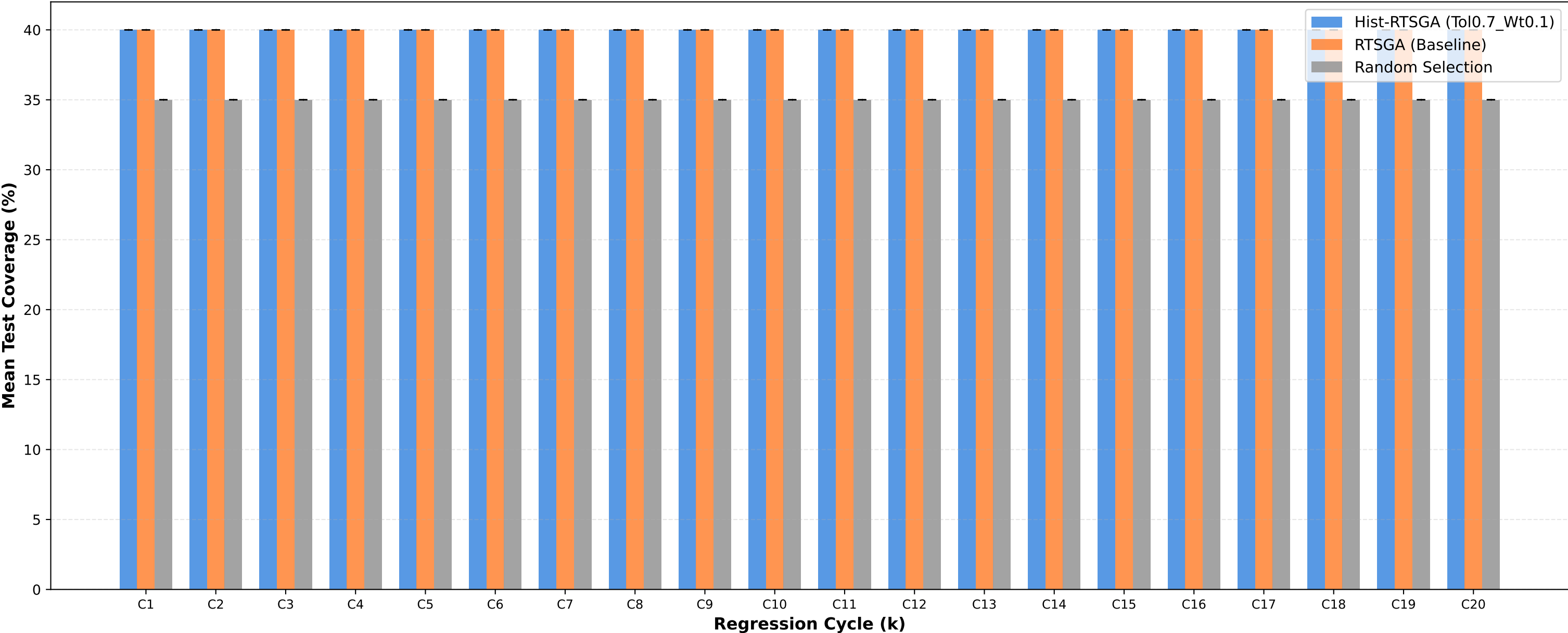
Test Coverage: Tol0.7_Wt0.1 vs RTSGA vs Random
