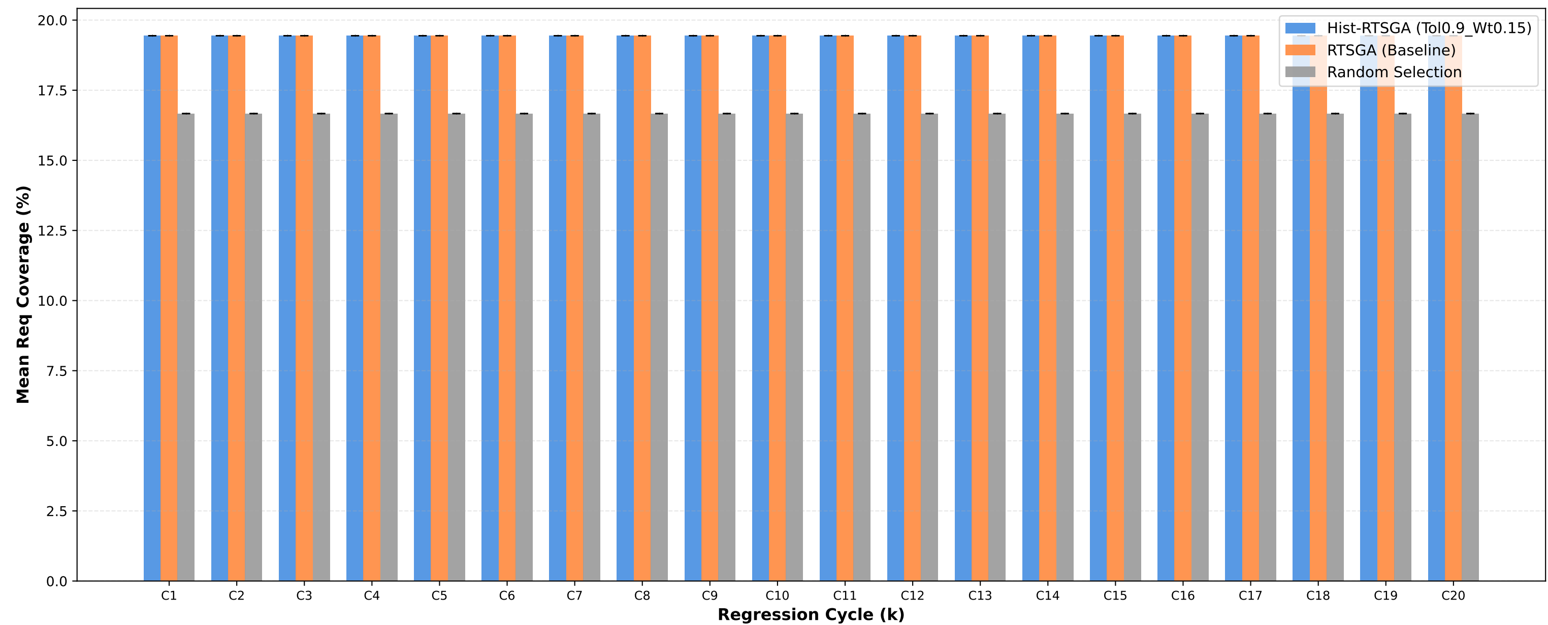
Req Coverage: Tol0.9_Wt0.15 vs RTSGA vs Random
